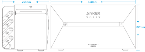
Figure: Anker SOLIX BP1600 Expansion Battery
